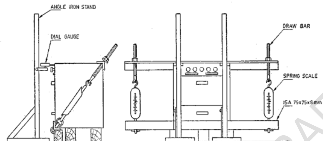
Figure A.1— Apparatus for determining strength of cooking range bodies showing set- up for testing end- frames
